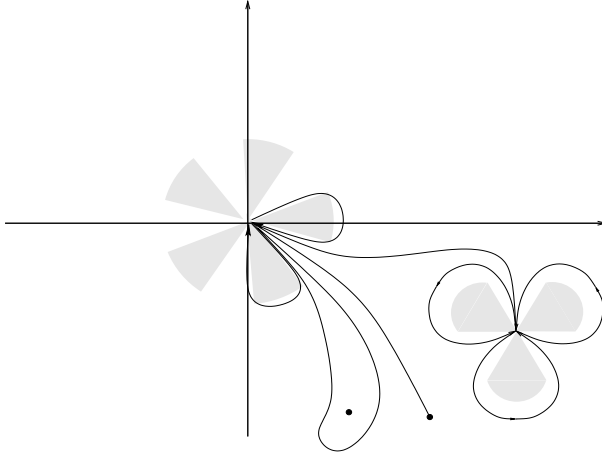
Figure 3: The contours \gamma_i , i \in I_L in the \omega plane.
